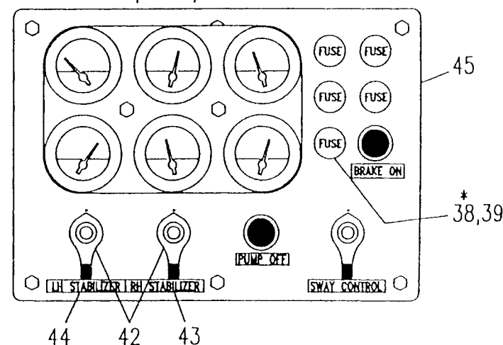
Option / Stabilizers
